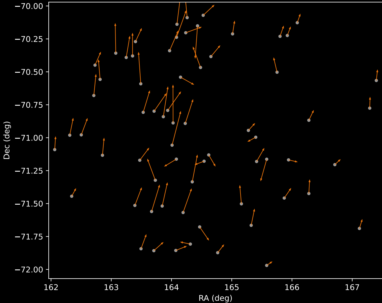
GALAH DR4 Cluster 2 Proper Motion Vectors (n=66)
