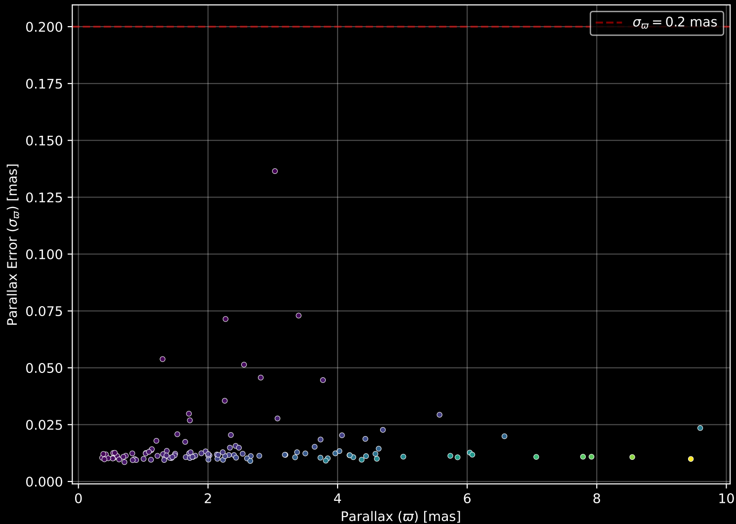
GALAH DR4 Field: [7207] Parallax Quality (n= 119)
