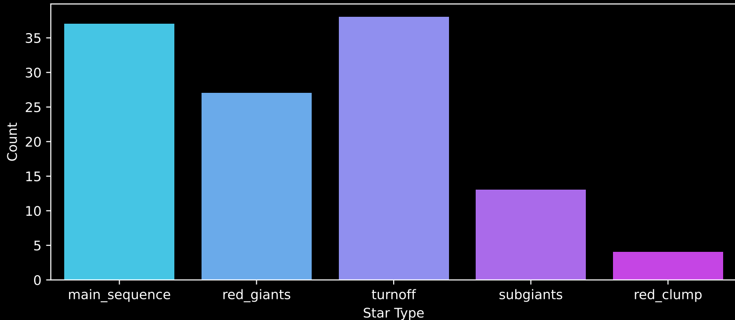
GALAH DR4 Field: [7207] Count plot of Star Type
