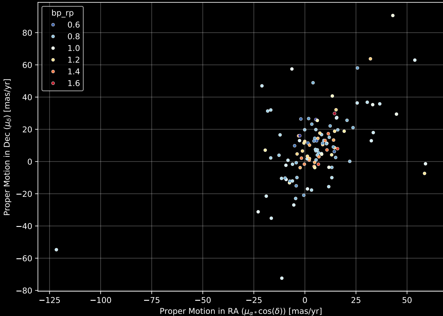
GALAH DR4 Field: [7207] Proper Motion Diagram (n= 119)
