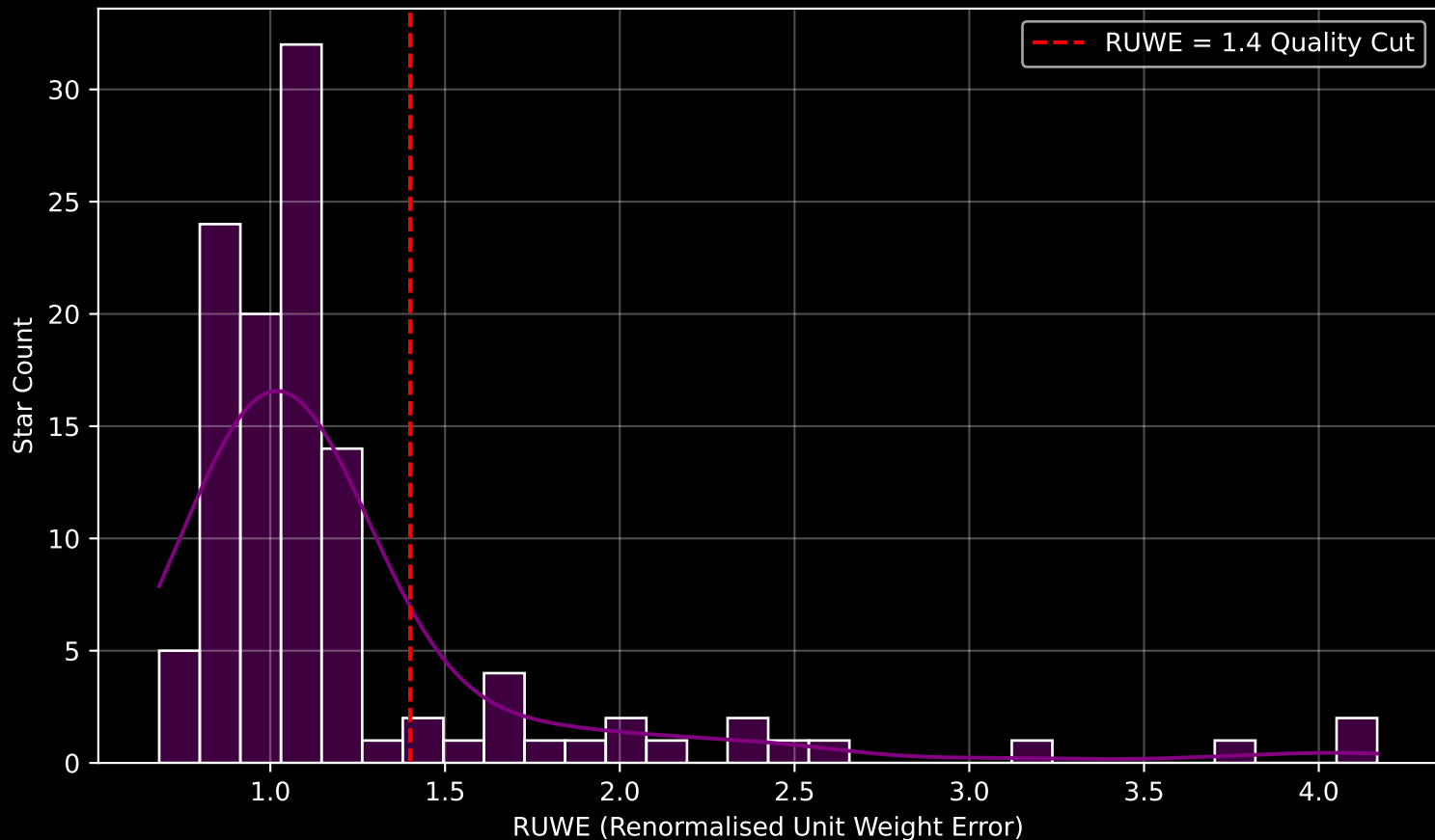
GALAH DR4 Field [7207] RUWE Distribution (n= 116)
